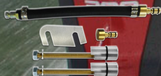
ASNU 185FIGHT Injector Fuel Connection & Blanking plug for Ficht
