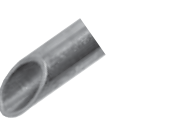
4500 Bowl Vent Tube (5/16" O.D. x 1.145 L)
