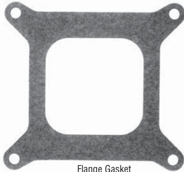
Flange Gasket (4160) (1 11 / 16 " bore) 20-2257 (3/64" thk.)
