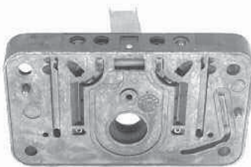
4779 Secondary Metering Block (4-Corner Idle)
