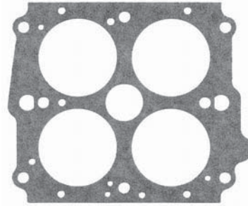
Throttle Body Gasket (4180) 20-2198 (108-57)
