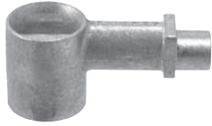
Straight Leg Booster H19-5 .125 orifice H19-35 .135 orifice (List 7448) H19-32 .144 orifice H19-56 Raw Casting (drill to size)
