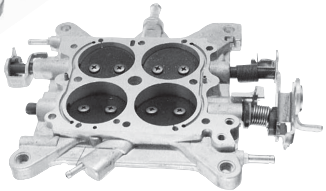
Base Plate w/ shafts (List 4779) H25-73 Four-Corner Idle (112-96)
