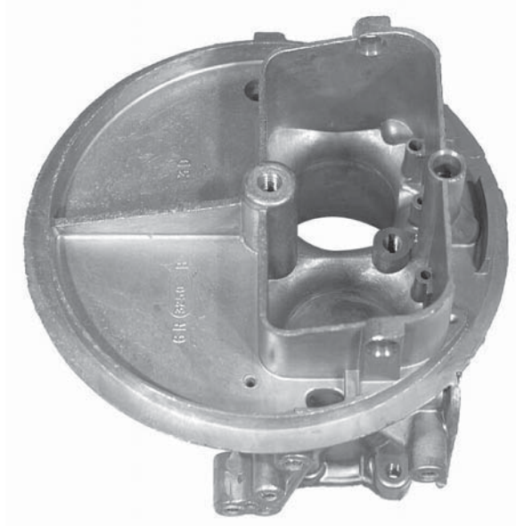
Main Body {Bare Machined} H25-94 350 / List 7448 H25-54 500 / List 4412
