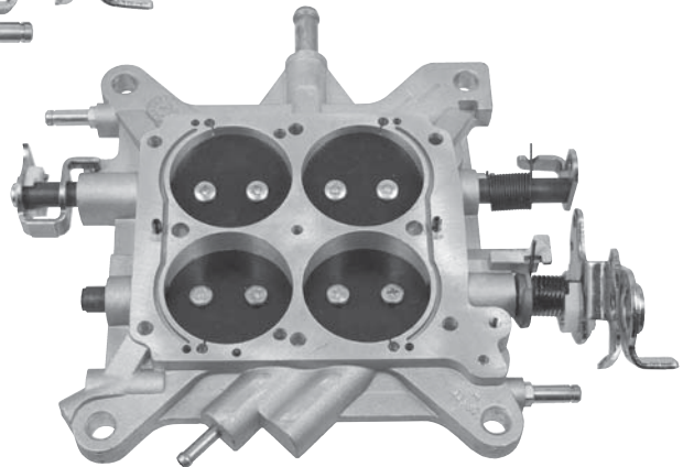
Base Plate w/ shafts (List 4781) H25-48 Four-Corner Idle (112-97)
