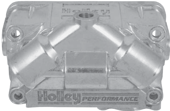
Aluminum V-Bowls w/Clear Sight Glass Installed (center hung)
