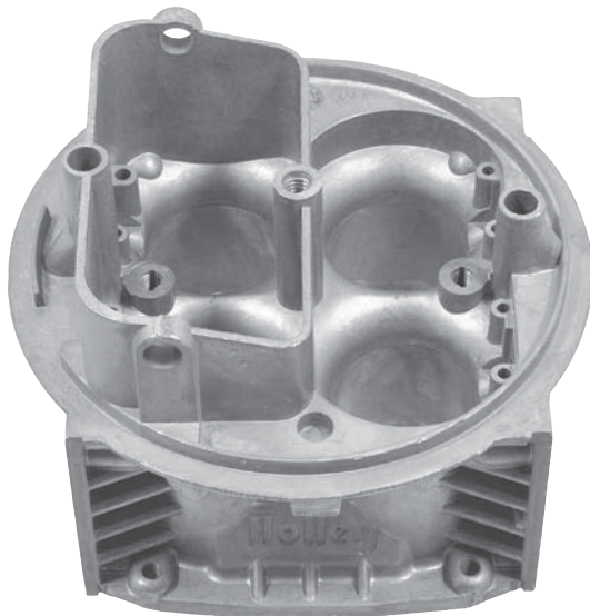
Main Body {Bare Machined} H25-98 650 / List 4777 H25-55 750 / List 4779
