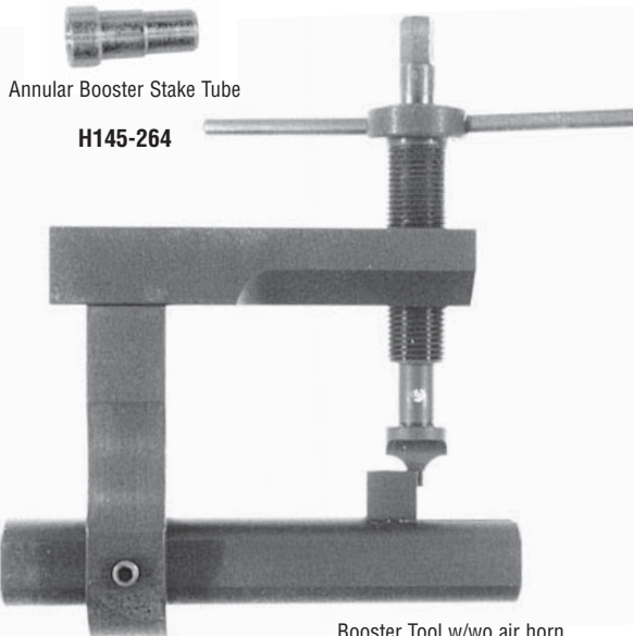
Booster Tool w/wo air horn RT-24 Replacement Cutter Tip RT-35
