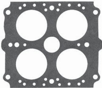
Throttle Body Gasket (17/16" x 17/16" bore) 20-1639 green fiber H20-271 black fiber (108-61)
