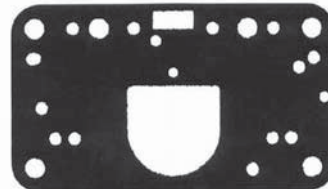
Metering Block Gasket
