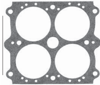
Throttle Body Gasket (111/16" x 111/16" bore) 20-1095 black fiber H20-273 black fiber (108-5)
