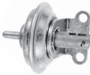
Choke Pull-Off 10-2107 (9-118)
