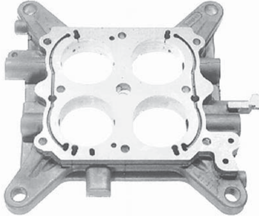
Base Plate w/o shafts H25-97 390 HP H25-114 830 HP H25-115 950/1000 HP H25-116 650/750 HP
